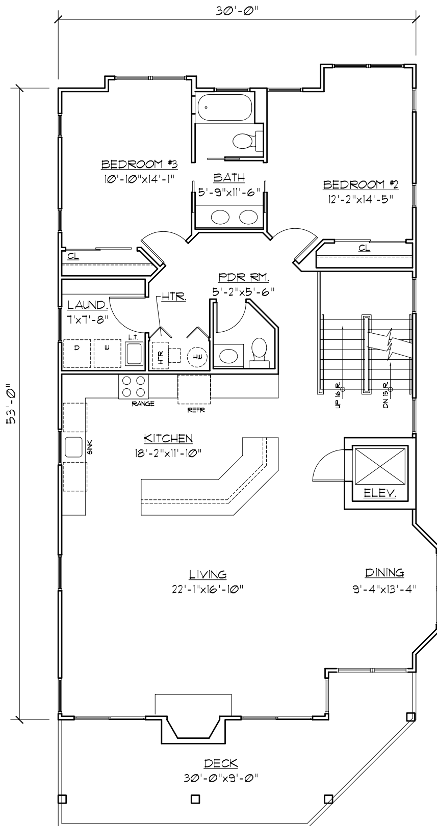
Second Floor Plan 1,602 S.F. of LIVING SPACE
