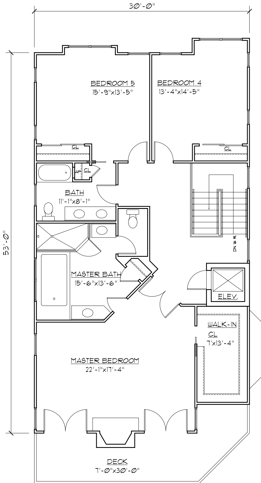
Third Floor Plan 1,505 S.F. of LIVING SPACE
